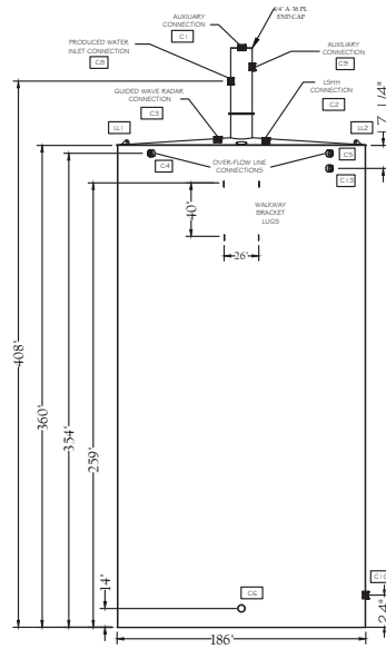
0° (TANK DETAIL)
