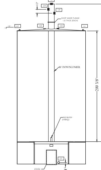
180° (GUNBARREL DETAIL)
